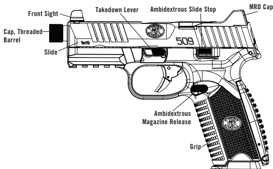
Left view of the FN 509 Tactical pistol (non-manual safety model shown).
